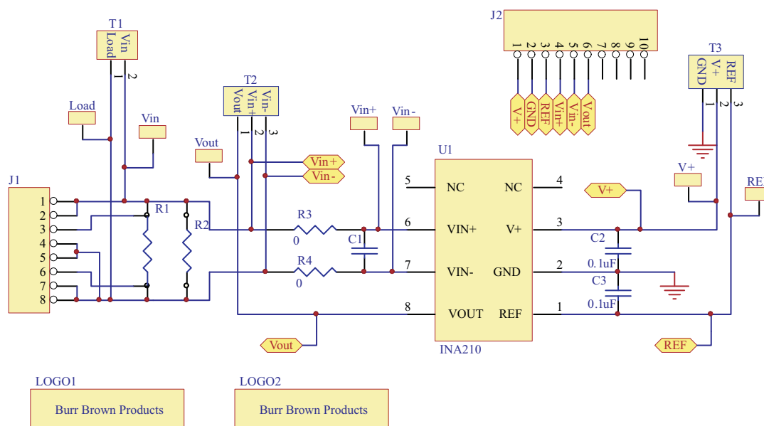
Figure 11. INA210-214EVM Schematic
