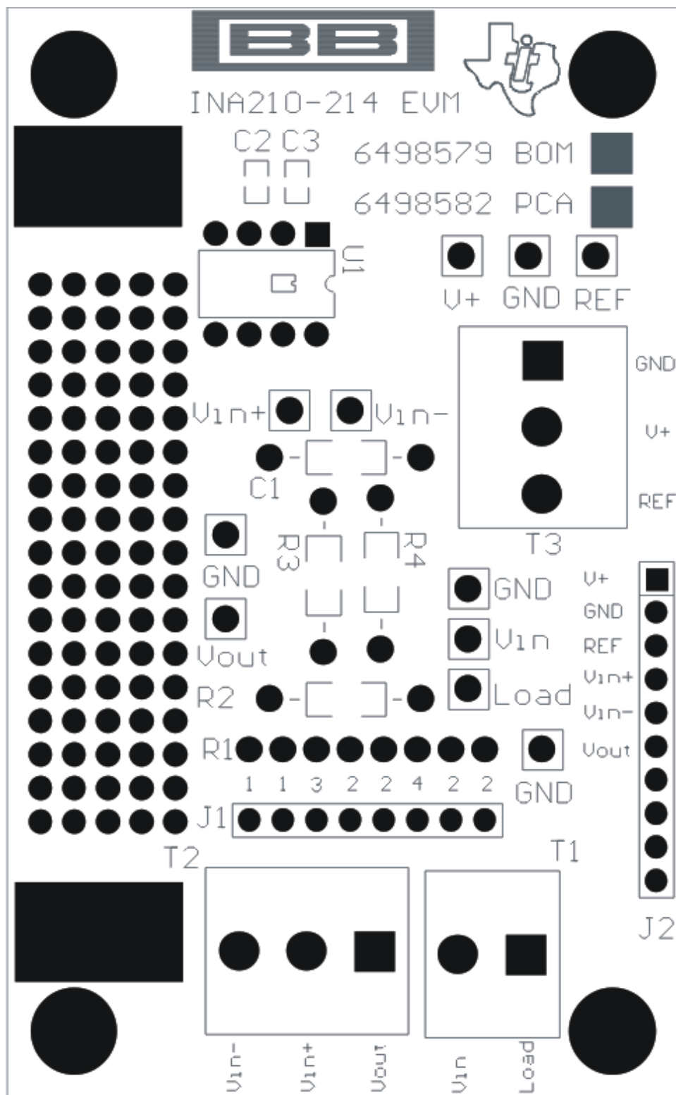
Figure 12. INA210-214EVM PCB
